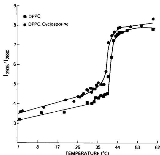
FIGURE 4 Raman intensity peak height intensity ratios I_{2935}/I_{2880} as a function of T for pure DPPC (■) and 10% CSA (●) bilayers. The increase in this ratio in the gel state for CSA-containing bilayers reflects an increased fraction of gauche conformers along the lipid acyl chains, as well as a small contribution from the CSA spectrum.
